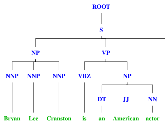
Fig. 2. Constituency parse tree example from Listing 9
