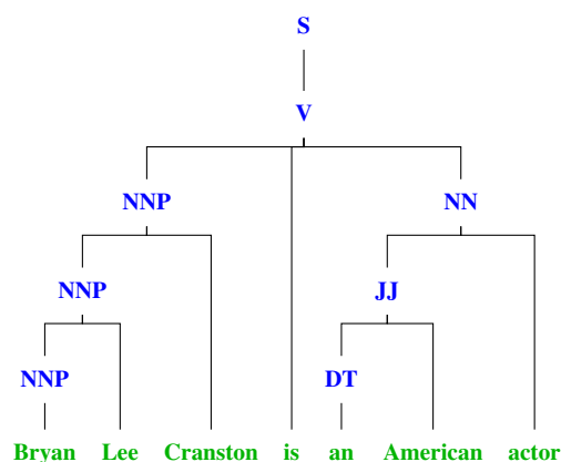
Fig. 3. Dependency parse tree example
