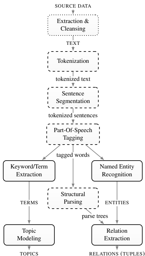
Fig. 1. Overview of a typical Information Extraction process. Dotted nodes indicate a preprocessing task, dashed nodes indicate a core NLP task and solid nodes indicate a core IE task. Small-caps indicate potential inputs and outputs for the IE process. Many IE process may follow a different flow to that presented here for illustration purposes (e.g., some Keyphrase Extraction processes do not require Part-Of-Speech Tagging).
